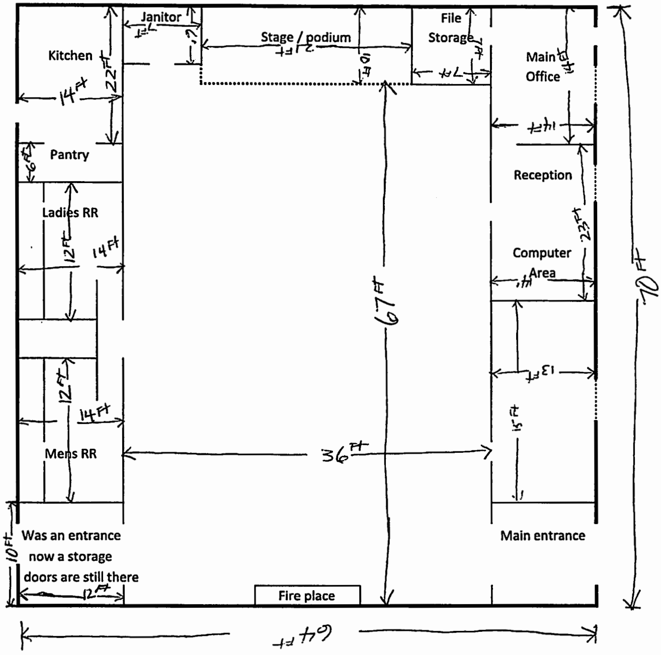
KLAGETOH CHAPTER'S CURRENT FLOOR PLAN
